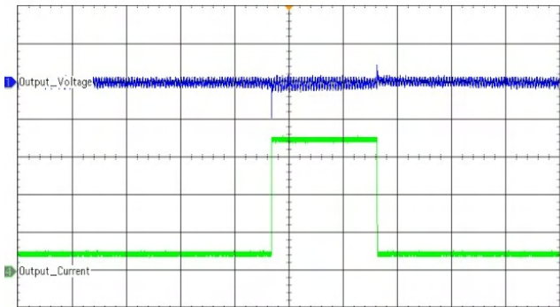
Figure 10. Load transient response: from 10% to 100% and from 100% to 10% at nominal output voltage (AC Coupled)
