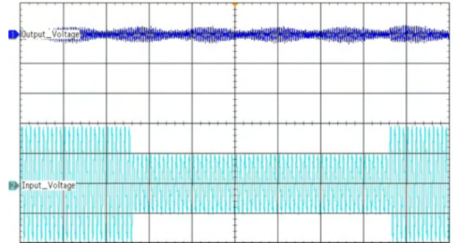
Figure 12. Line transient response: from 265 V RMS to 135 V RMS and from 135 V RMS to 265 V RMS at nominal output voltage (AC Coupled)
