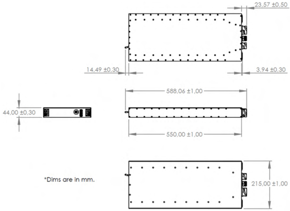
Figure 20. Mechanical Dimensions
