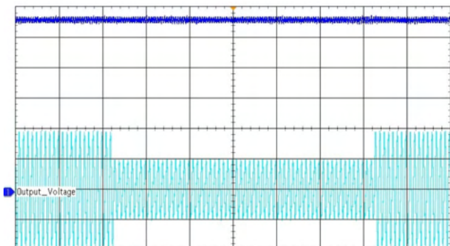
Figure 11. Line transient response: from 265 V RMS to 135 V RMS and from 135 V RMS to 265 V RMS at nominal output voltage (DC Coupled)
