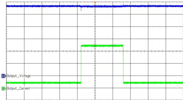
Figure 9. Load transient response: from 10% to 100% and from 100% to 10% at nominal output voltage (DC Coupled)
