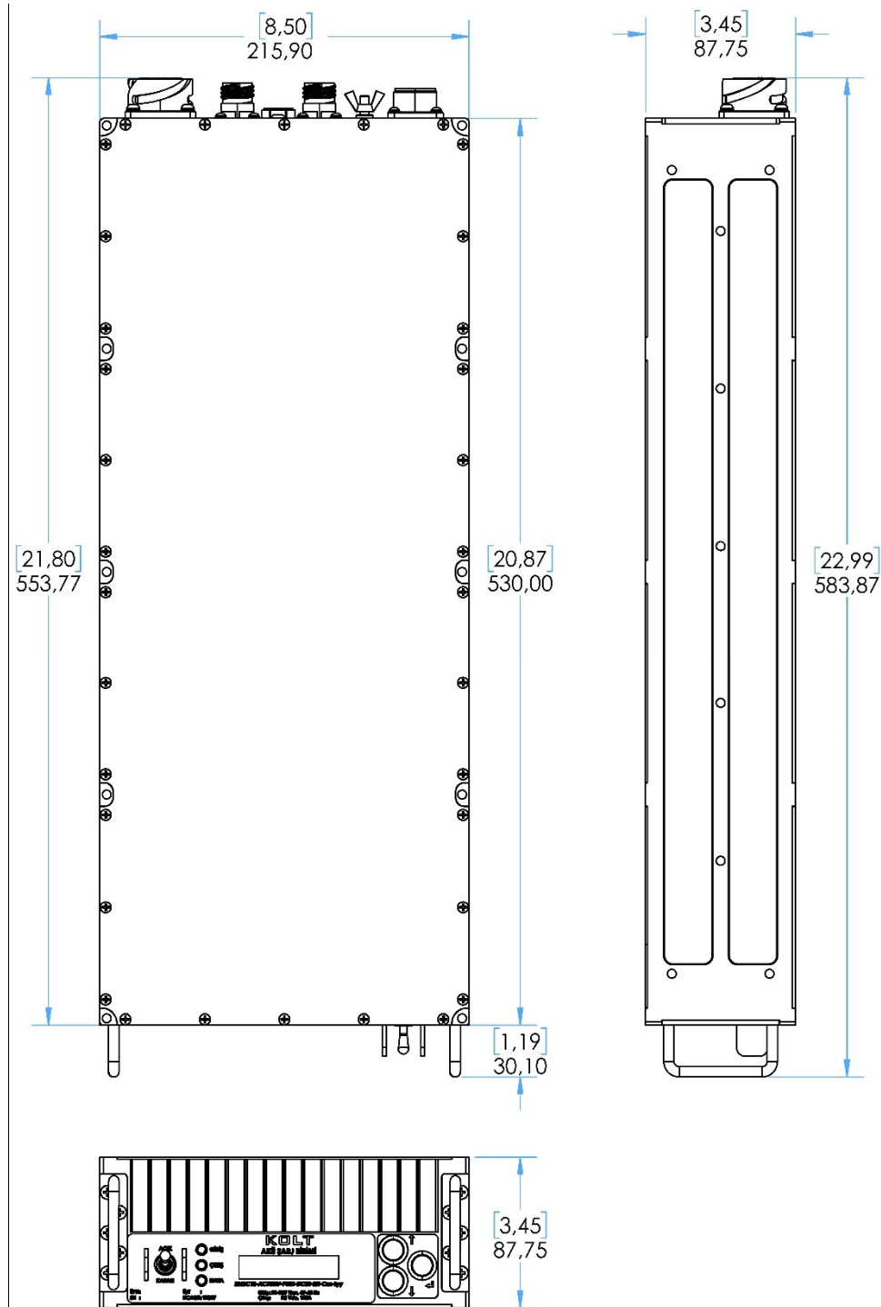
Figure 28. Mechanical Dimensions
