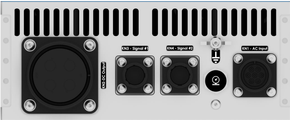
Figure 18. Connector Panel
