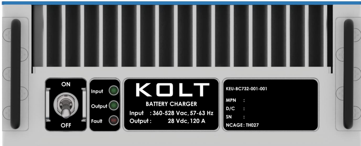
Figure 17. Connector Panel
