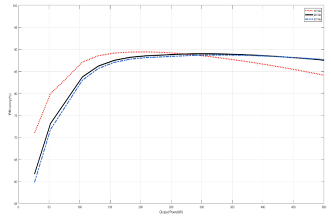
Figure T. Efficiency versus output power at minimum, nominal and maximum input voltage
